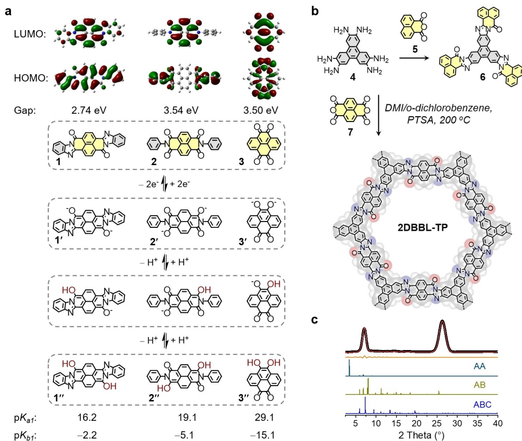
Figure 1. Design of active sites. (a) Electronic structures and proposed electron-transfer processes for model compounds 1 , 2 , and 3 . (b) Schematic synthesis of perinone-based 2DBBL-TP . (c) Experimental (red) and refined (black) as well as the calculated PXRD patterns of 2DBBL-TP .
